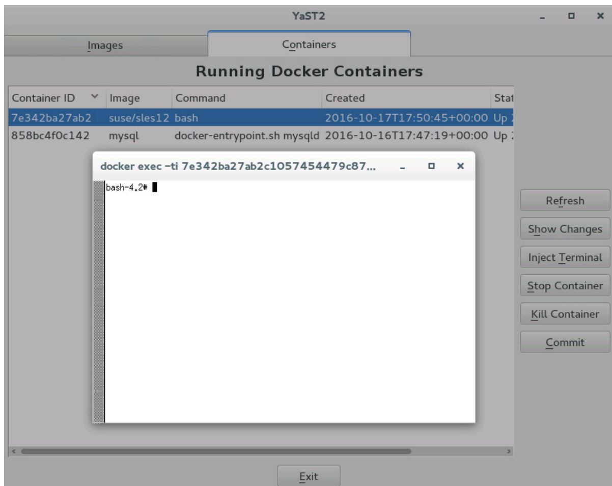
FIGURE 3. SUSE Enterprise Linux 12 uses YaST for most administrative tasks, and the yast2-docker module offers a graphical way to manage containers, including injecting a terminal to anything that's running.
