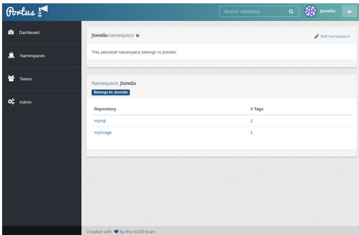
FIGURE 7. A running version of Portus provides a clean graphical interface, plus security and other features, to the locally installed docker-registry. The repository contains two images ready for sharing.
