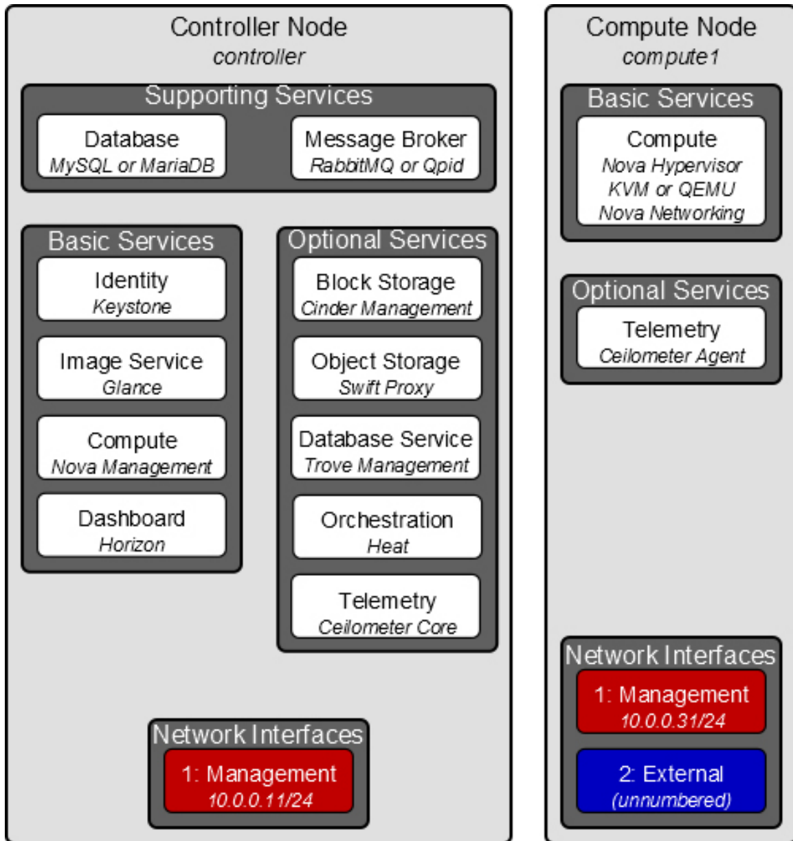
FIGURE 1. OpenStack Architecture Diagram (image from http://docs.openstack.org/icehouse/install-guide/install/apt/content/ch_overview.html#architecture_example-architectures )
