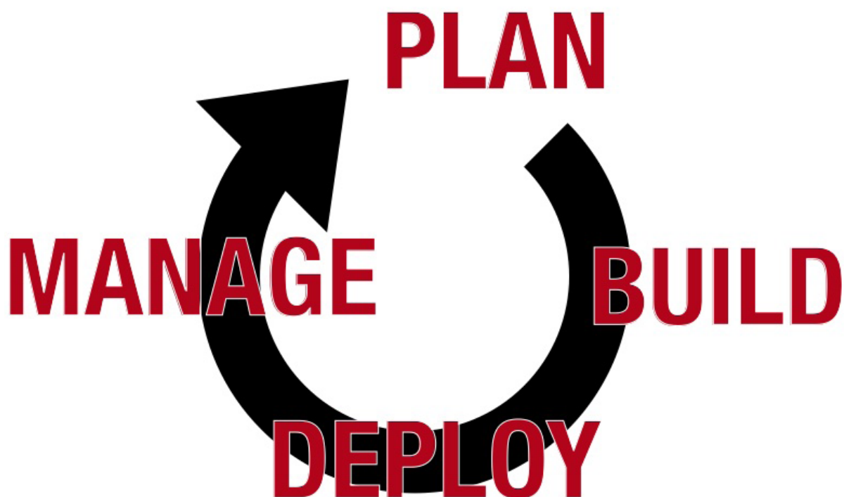
FIGURE 3. API Lifecycle
