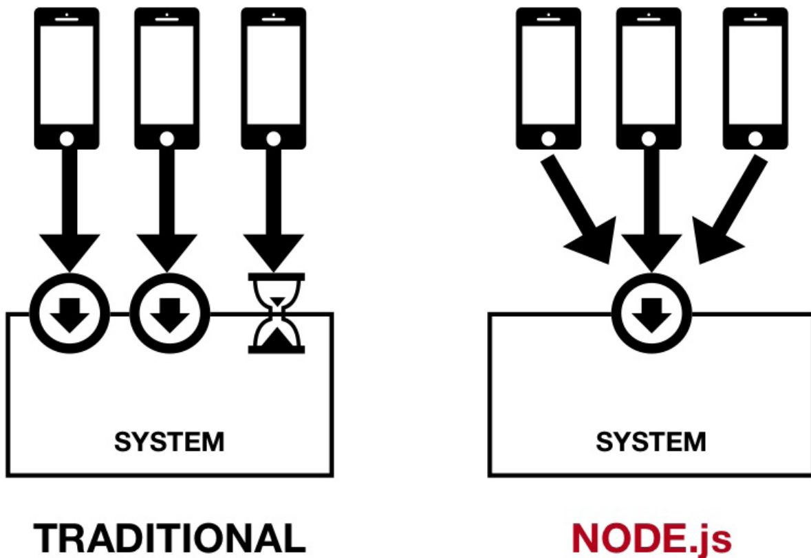
FIGURE 4. Node.js
