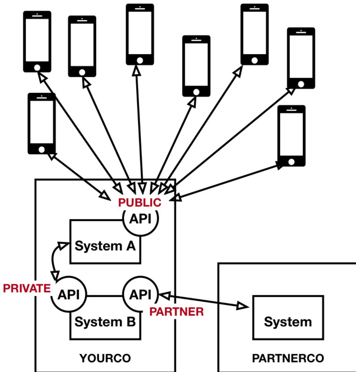
FIGURE 2. API Types
