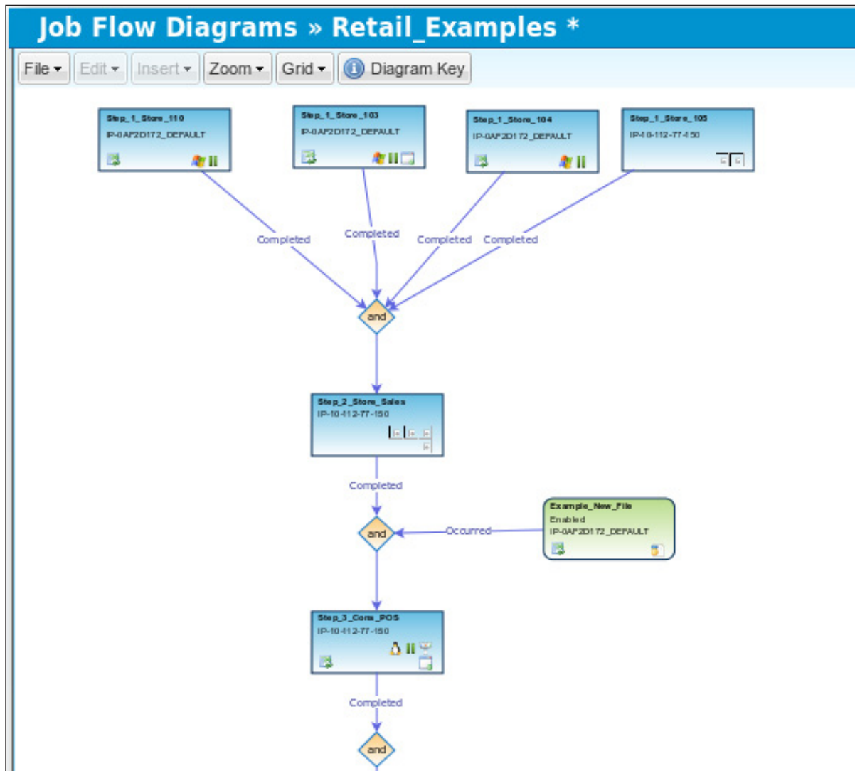
FIGURE 4. Job flow diagrams make process dependencies easy to understand. Role-based diagrams provide different stakeholders with the information they need.
